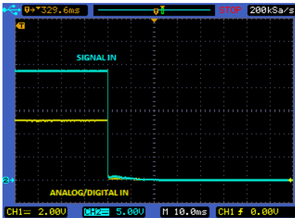
Analog/Digital Input Turn-off
