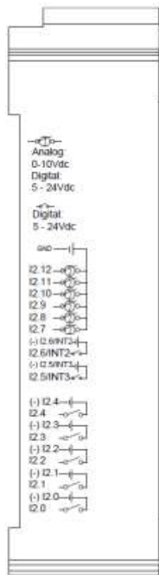
Analog/Digital Inputs
