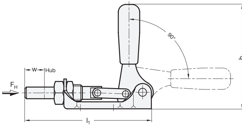
2 Form AS Grundkörper Stahlblech
